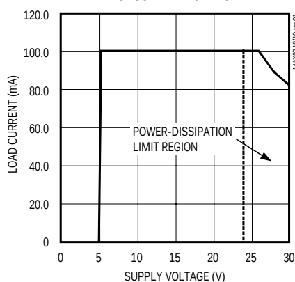
SAFE LOAD-CURRENT OPERATING AREA vs. SUPPLY VOLTAGE
